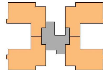
CLUSTER {B,C,D}
